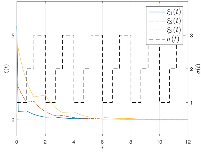
Fig. 4. The state response with the time-dependent switching signal.
